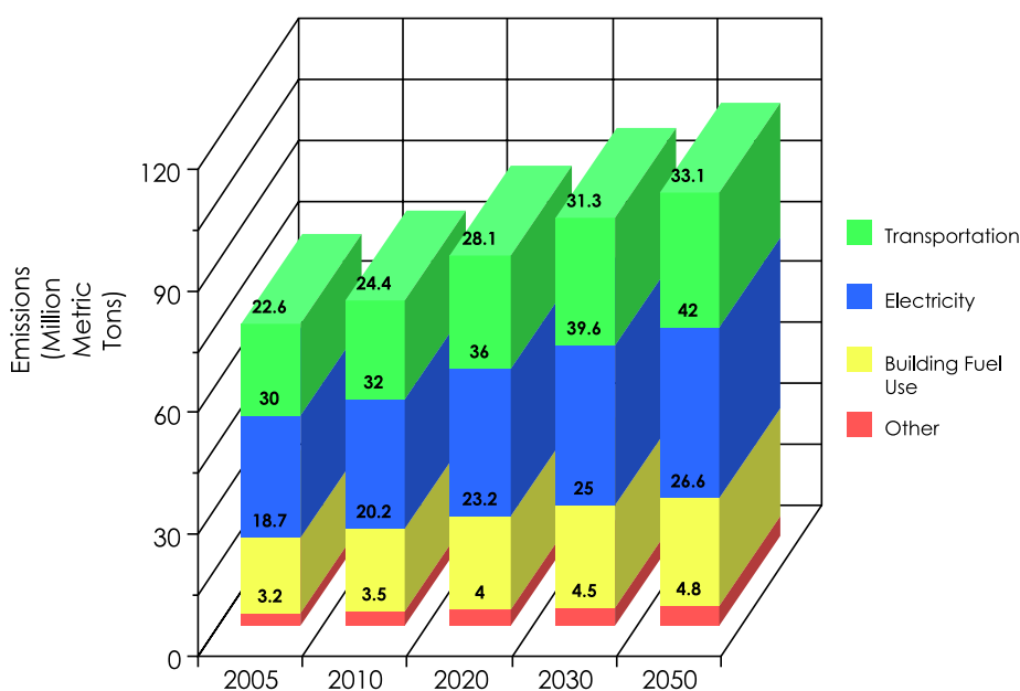
CO 2 Emissions Projections for Metropolitan Washington (2005-2050)
