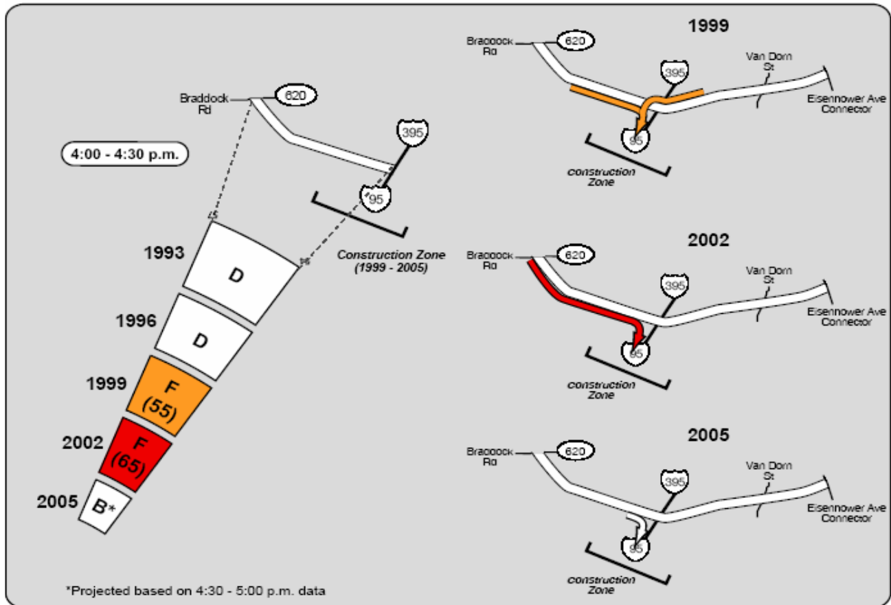
Figure 5: Improved conditions on I-495 Outer Loop (Fairfax County)
