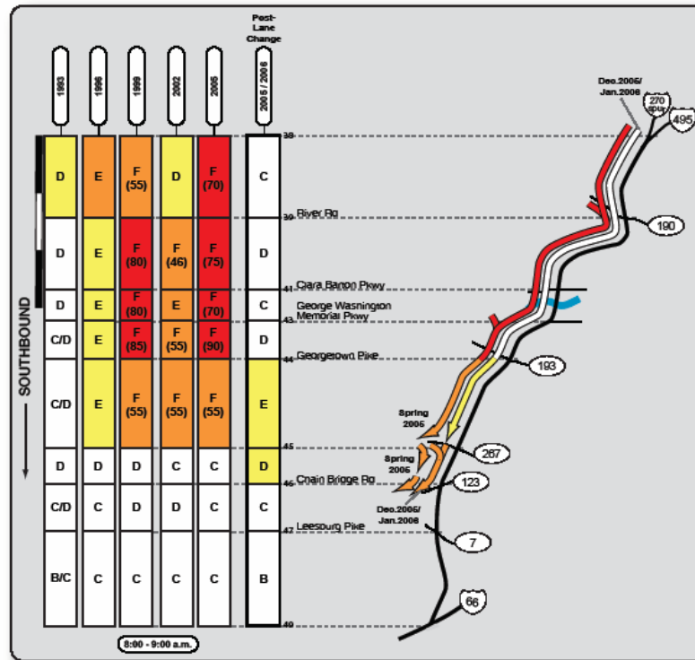
Figure 6: I-495 (Outer Loop) Improvement in Congestion (Morning)
