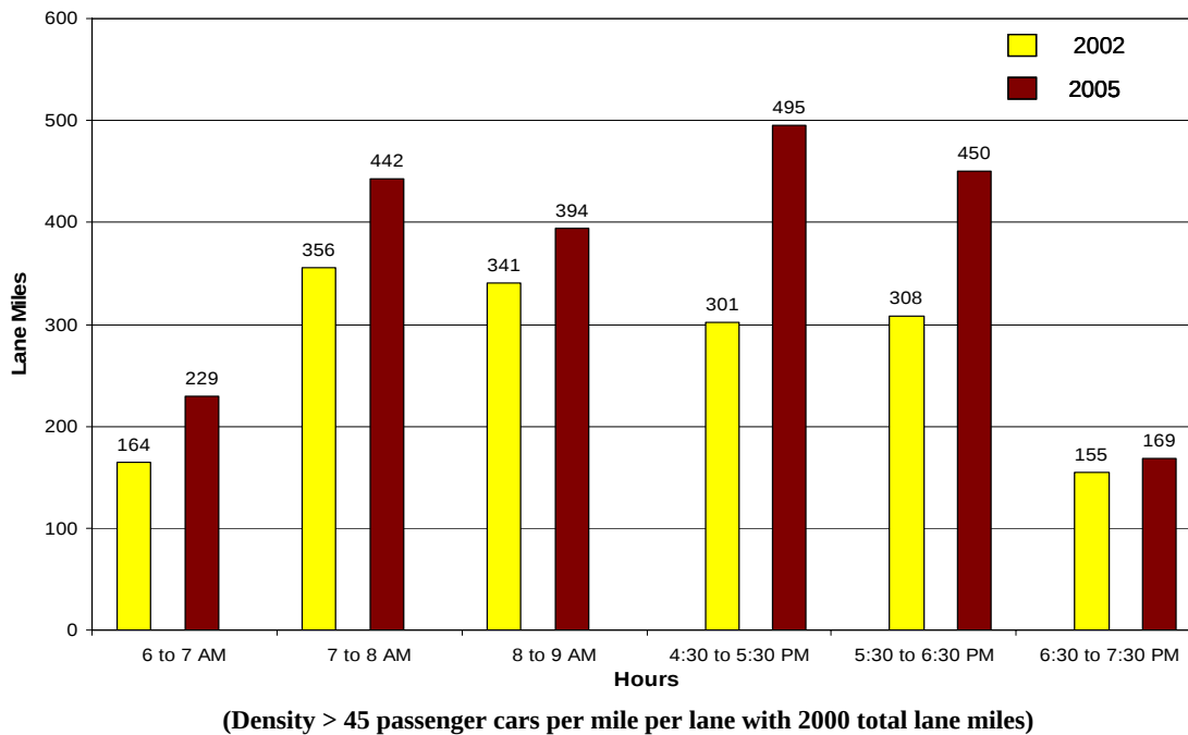
Figure 3: Lane Miles at LOS F - 2002 and 2005
