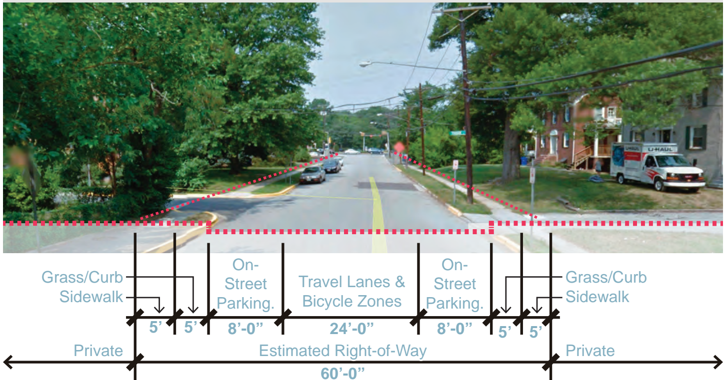
FIGURE 44 | GUILFORD ROAD (STREET VIEW AND SECTION)
