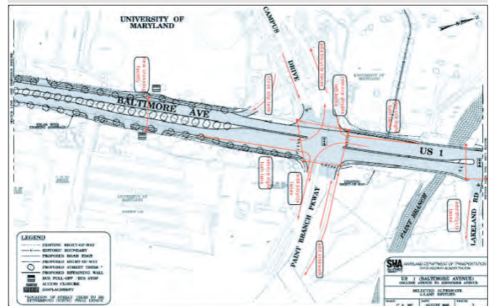
FIGURE 7 | US 1 & PAINT BRANCH PKWY ALTERNATIVE EXAMPLE
