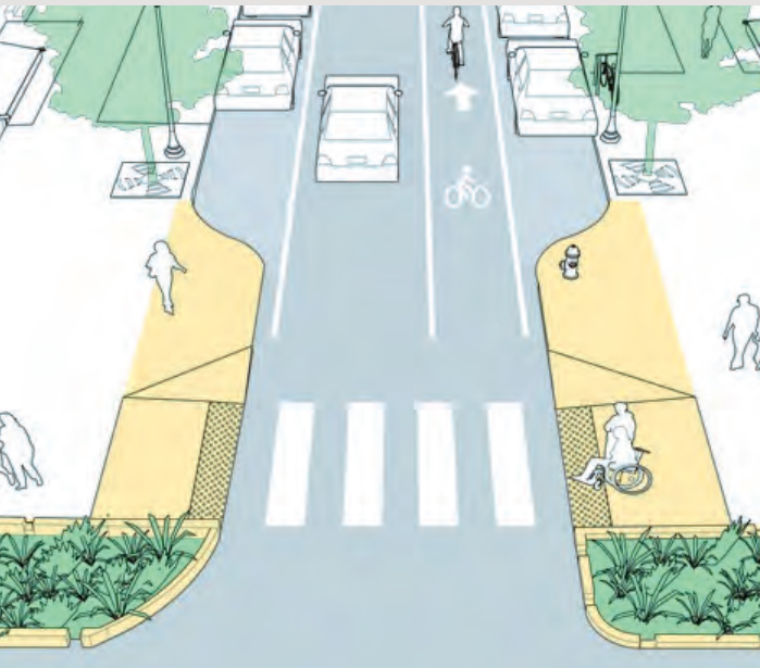
The above image combines parking, curb extensions and bike lanes to narrow the street and slow motor vehicles. | Source: NACTO
