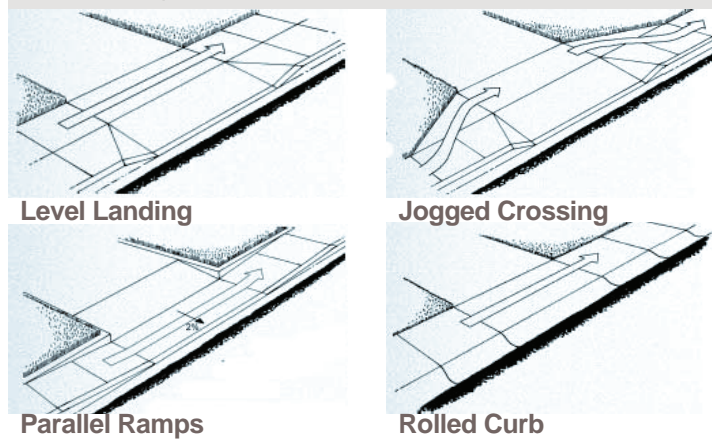
FIGURE 75 | DRIVEWAY CROSSINGS
