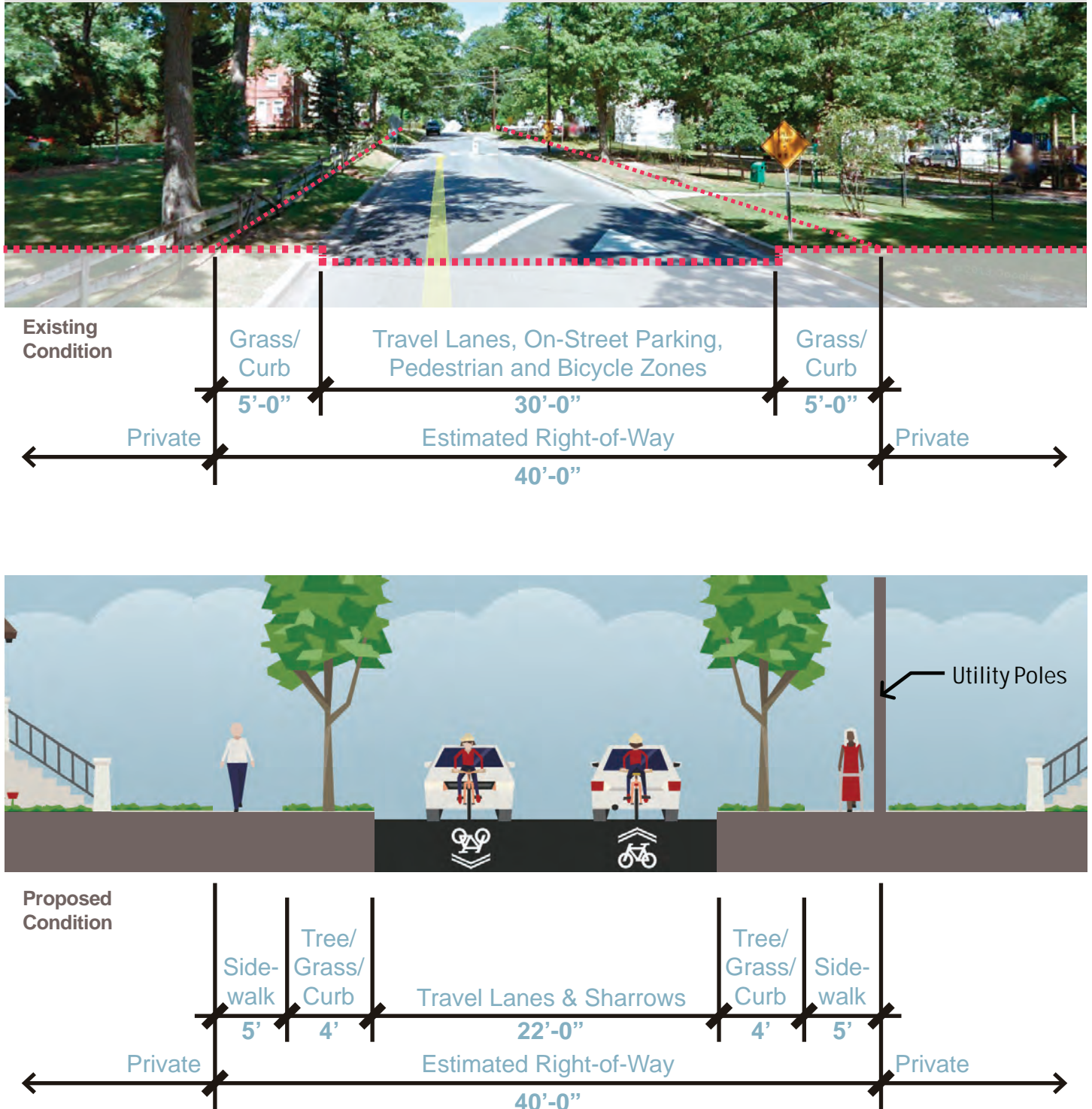
FIGURE 77 | HOLLYWOOD ROAD: EXISTING AND PROPOSED CONDITIONS
