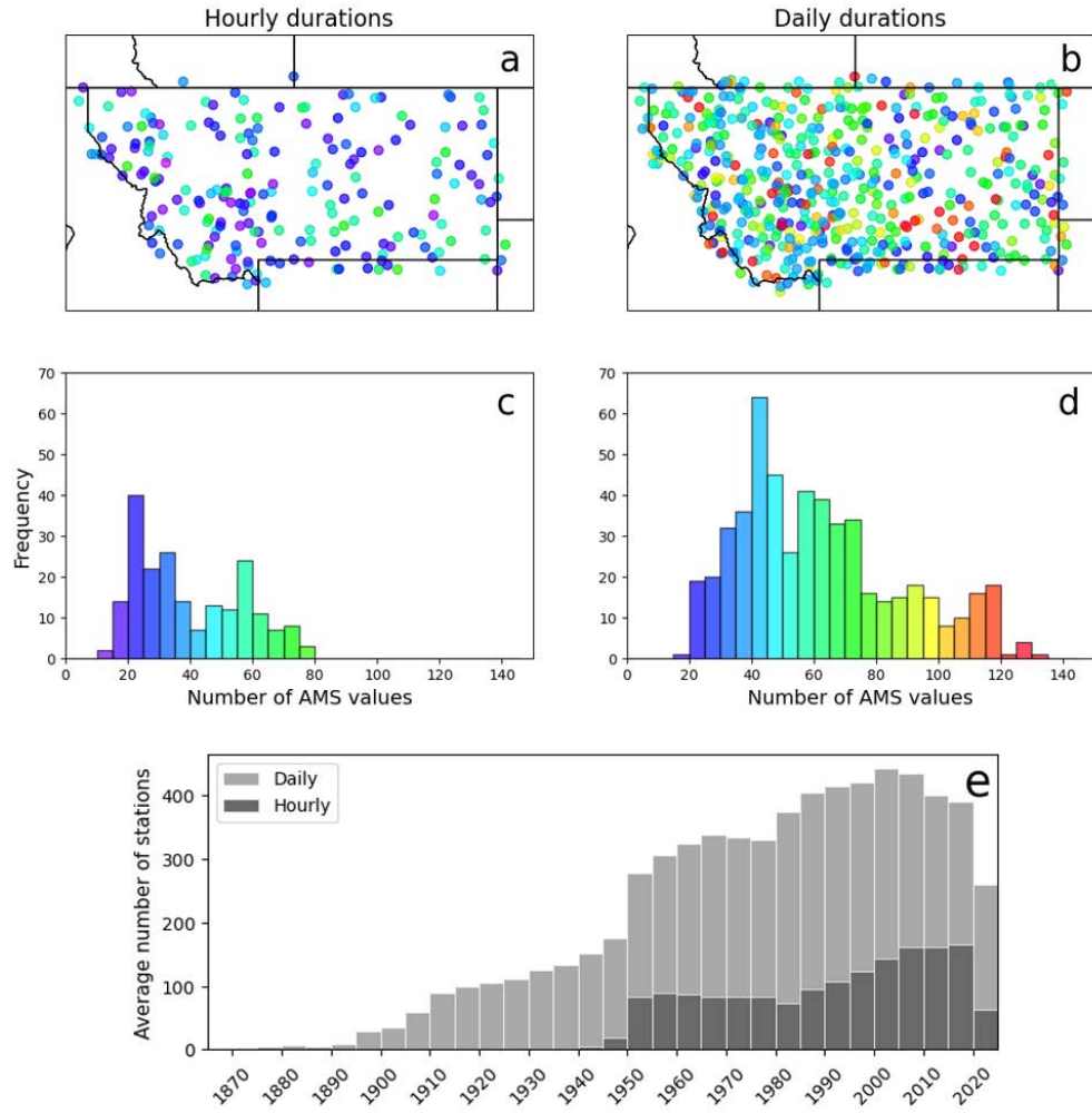
Figure 3. Station locations and histograms illustrating the number of AMS values per station for hourly (a,c) and daily (b,d) durations, and the number stations per year within this domain averaged over 5-year periods (e).
