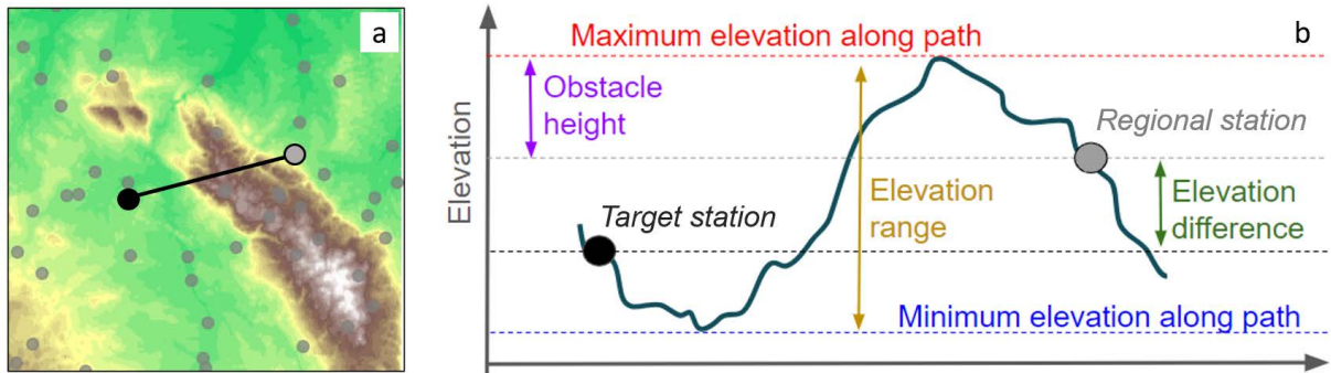
Figure 4. Definition of elevation attributes along a path between a target station (black dot) and regional station (gray dot) as depicted from above (a) and as a cross-section (b).
