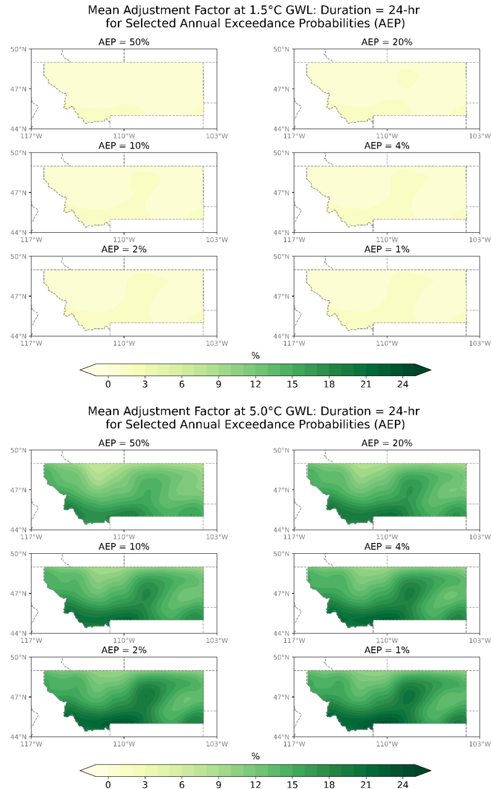
Figure 15. Atlas 15 Volume 2 adjustment factors for 24-hr duration and a range of AEPs under GWLs of 1.5°C (top) and 5°C (bottom). These adjustments are with respect to the current level of global warming relative to 1851-1900, which is 1.1°C. Thus, these adjustments are for further warming of 0.4°C and 3.9°C.
