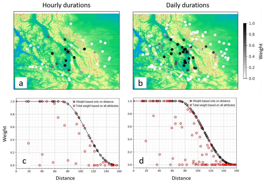
Figure 6. Example of regional weighting for hourly (a and c) and daily (b and d) durations, with the upper-bound determined by the distance weight (black points in c and d). Black dots in panels a and b show regional stations that contribute the most to estimations at the target station (encompassed by a black square), gray dots show stations with weights between 0 and 1, and white dots indicate stations with zero weight.
