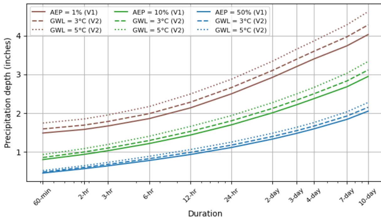
Figure 18. Atlas 15 depth-duration-frequency curves for selected durations and AEPs at Helena, MT (112.0 W, 46.6 N) for Volume 1 (present) and Volume 2 (GWL = 3°C and 5°C).
